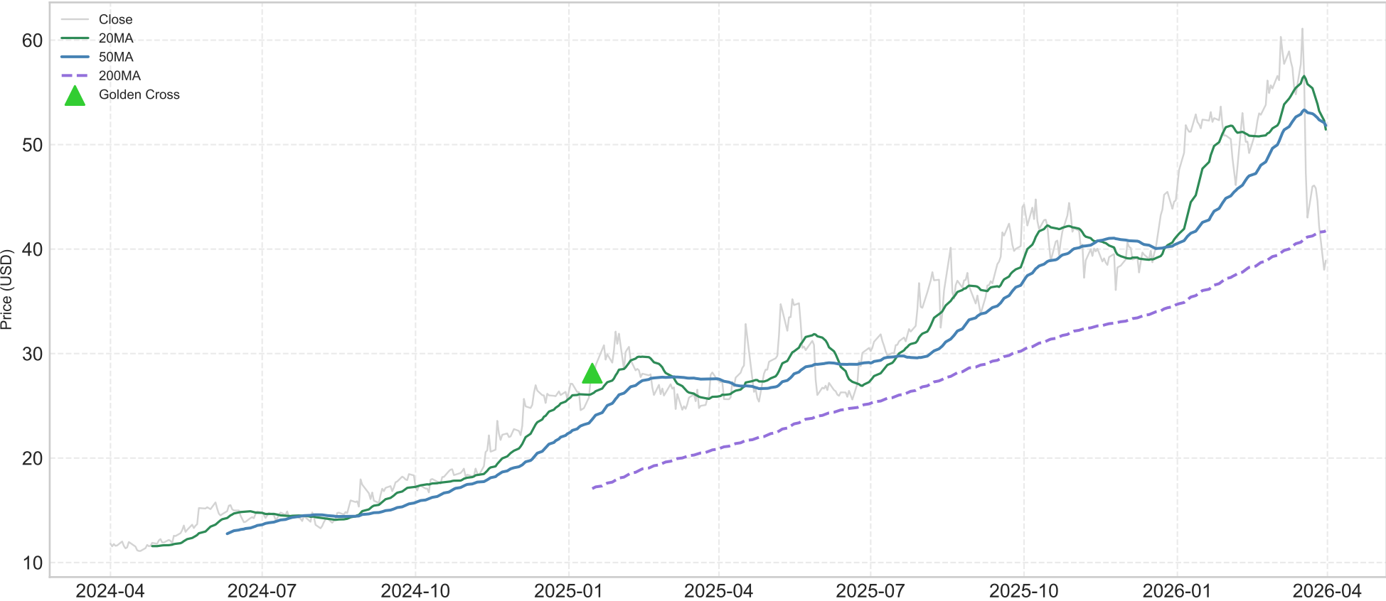
TATT — 2-Year Price with MAs & Crossover Signals
