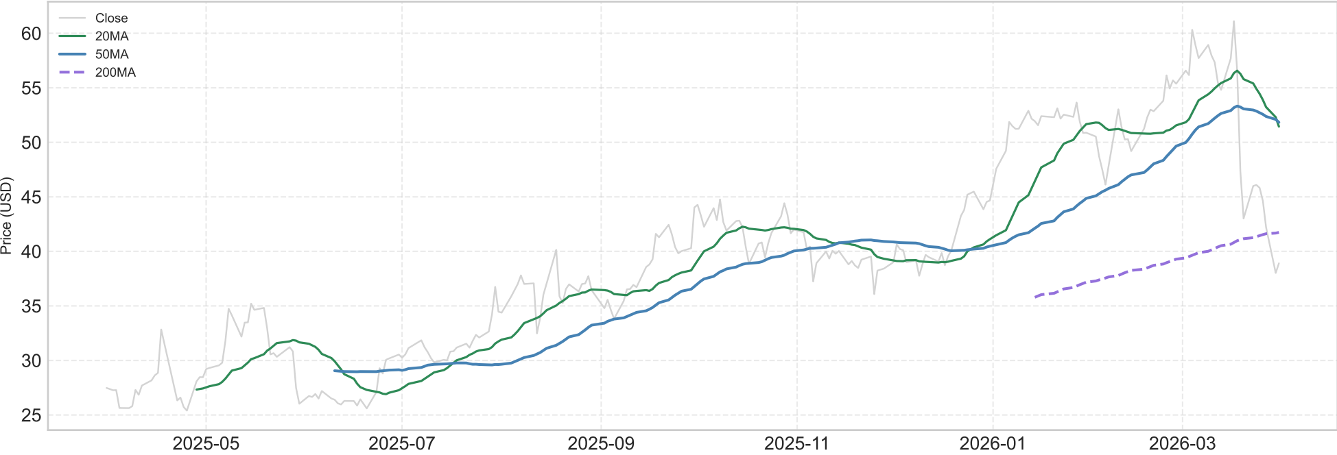
TATT — Closing Price with Moving Averages (1 Year)
